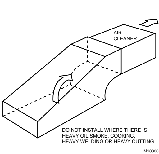
Fig. 11. Connecting air cleaner directly to a canopy hood with a minimum air entrance velocity of 120 fpm.
